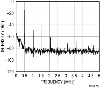
Figure 4. V_{OUT} Noise Spectrum ( V_{IN} = 48V , V_{OUT} = 24V at 3A)
