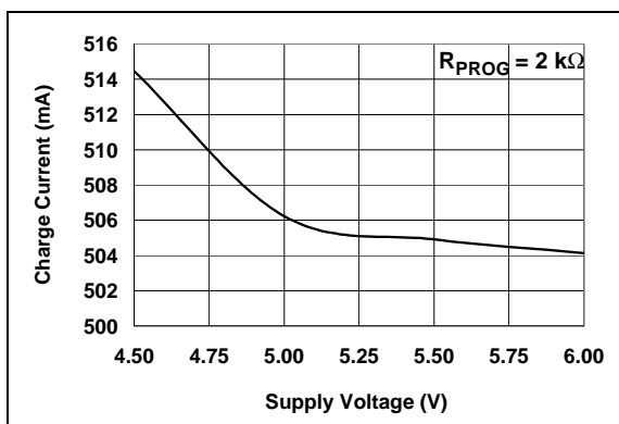
FIGURE 2-6: Charge Current ( I_{OUT} ) vs. Supply Voltage ( V_{DD} ).
