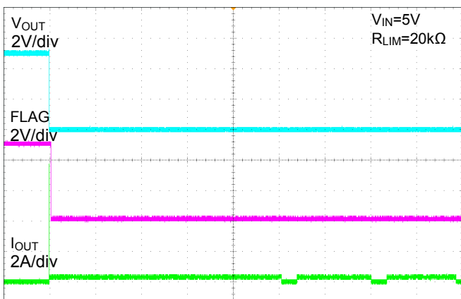
Figure 7. Extended Short-Circuit into Thermal Cycles
