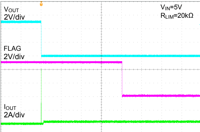
Figure 6. Short-Circuit Current Limit Response
