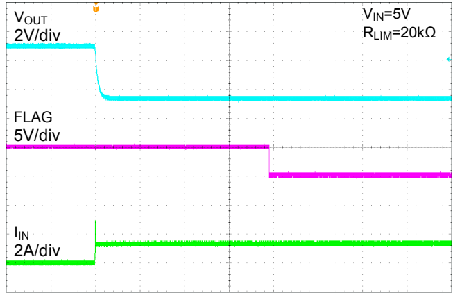
Figure 5. No Load to 1Ω Transient Response
