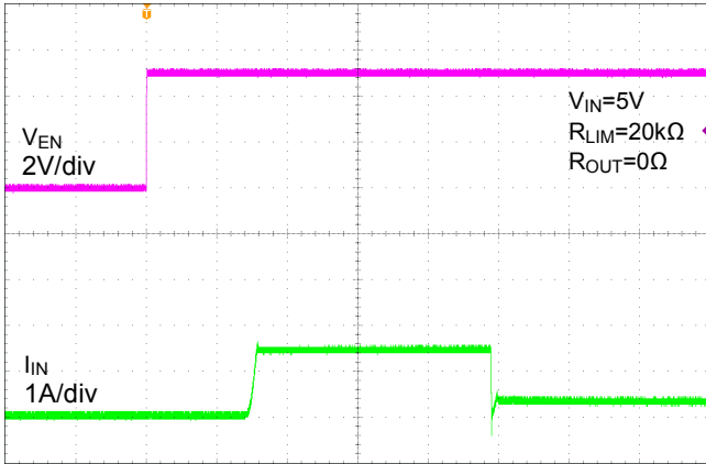
Figure 4. Device Enabled into Short-circuit
