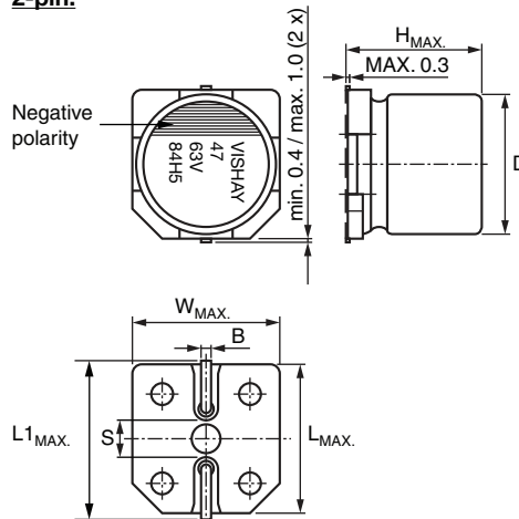
Fig. 2 - Dimensional outline
