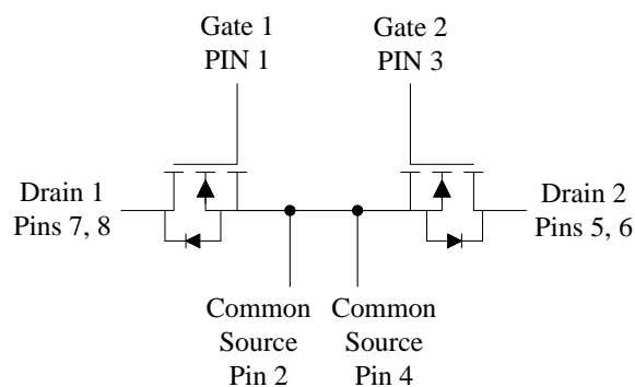
Circuit Image
