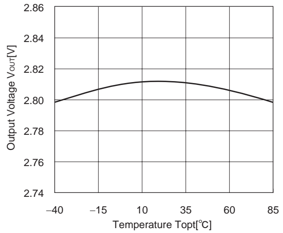
R1180x281x ( V_{IN}=3.8V )
