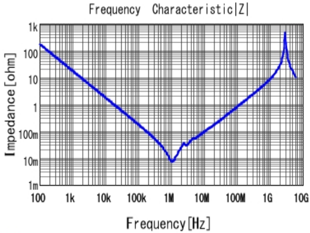
■ KCM55TR72A106MH01 |Z| DCOV, 25degC
