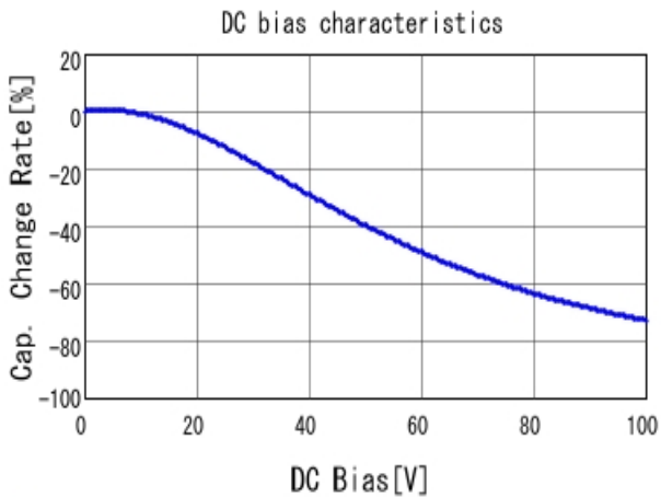
■ KCM55TR72A106MH01 C-DC bias capchange, 25.0degC, AC1V
