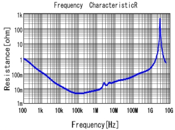
■ KCM55TR72A106MH01 R DCOV, 25degC
