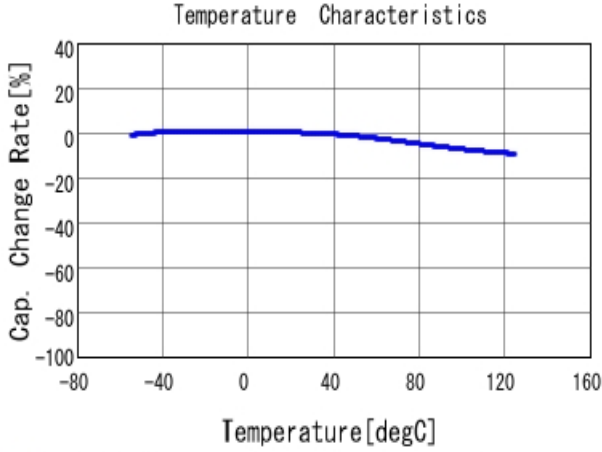
■ KCM55TR72A106MH01 C-Temp. capchange, DCOV, AC1Vrms
