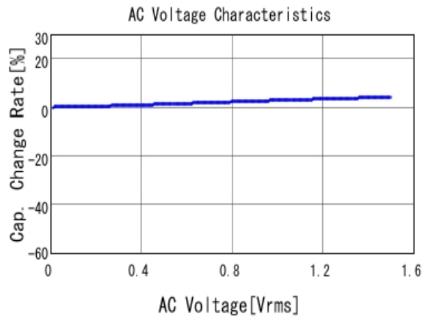
■ KCM55TR72A106MH01 C-AC Voltage capchange, DCOV, 25.0d
