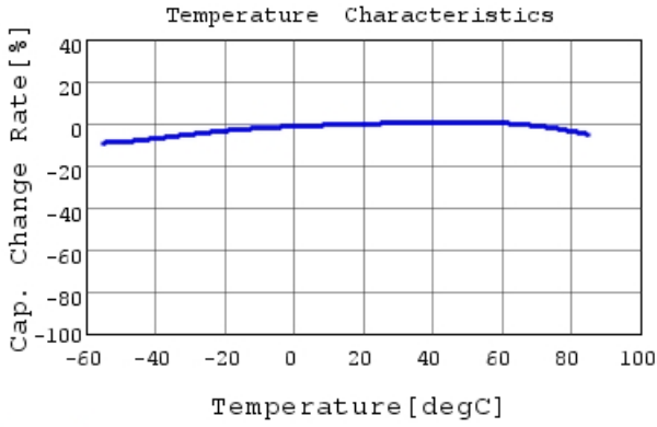
GRM31CR61H106KA12 C-Temp. capchange, DC0.0V,
