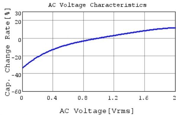
GRM31CR61H106KA12 C-AC Voltage capchange, Dc
