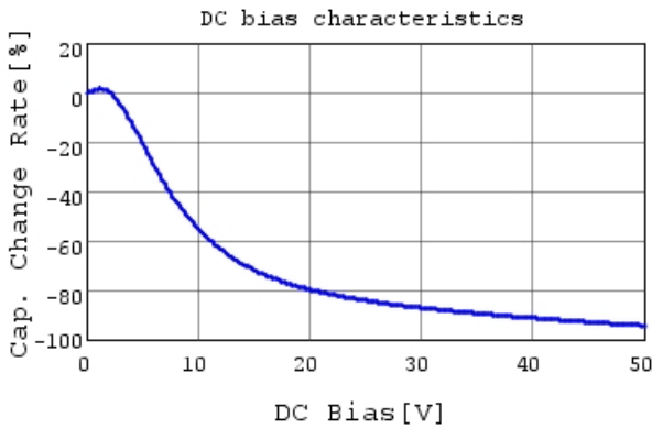
GRM31CR61H106KA12 C-DC bias capchange, 25.0c
