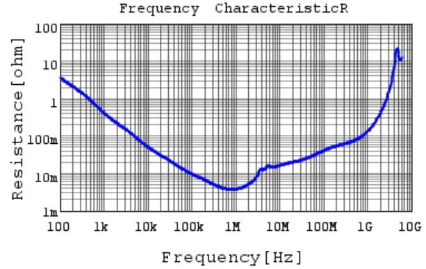
GRM31CR61H106KA12 R DCOV,25degC
