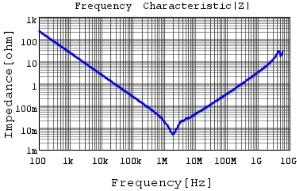
GRM31CR61H106KA12 |Z| DCOV,25degC
