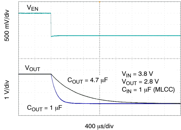
Figure 51. Enable Turn-off
