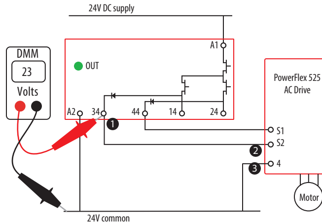
Figure 78 - Typical Connections to PowerFlex Drive
