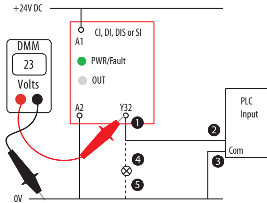
Figure 84 - Measure Y32 Voltage
