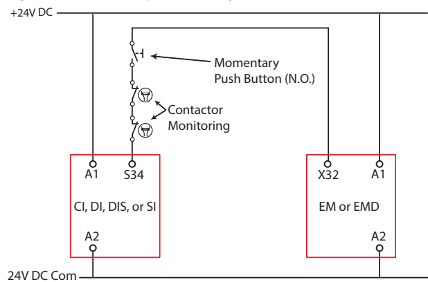
Figure 24 - Monitor Expansion Relay
