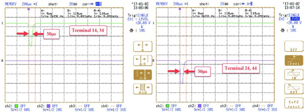
Figure 81 - OSSD Channel Transistor Test Pulse
