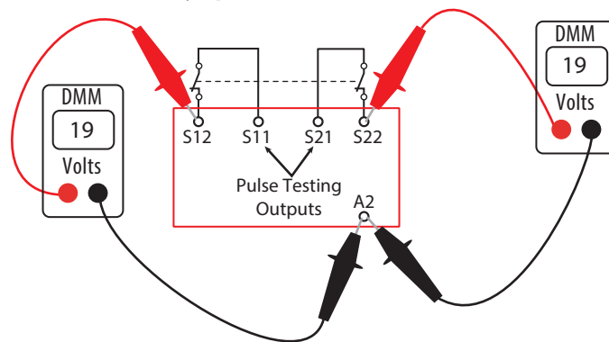
Figure 61 - Check the CI Safety Inputs with the Device Contacts Closed
