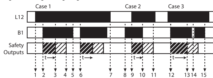
Figure 35 - Jog Timing Diagram
