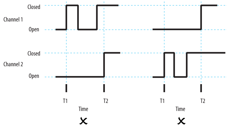
Figure 69 - Multiple Cycles on One Channel Are Not Allowed
