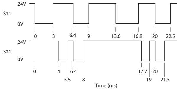
Figure 29 - Pulse Test Sequence for DI, DIS, and SI Safety Relays
