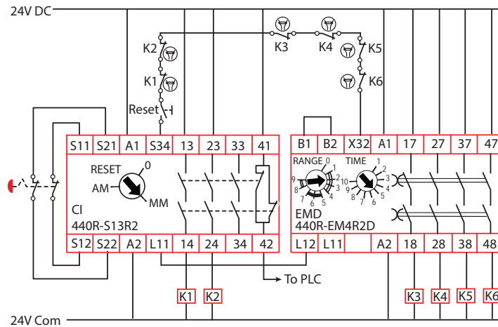
Figure 49 - EMD - Off Delay
