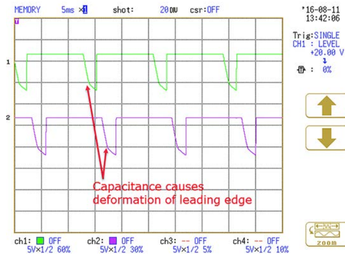
Figure 66 - Capacitive Effect on Pulse Tests
