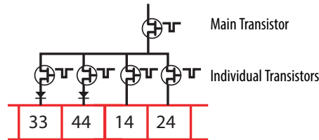
Figure 30 - Output Transistor Arrangement
