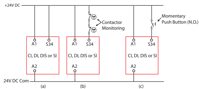
Figure 21 - Automatic/Manual Reset Connections
