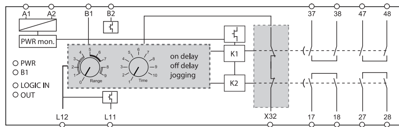
Figure 40 - EMD Safety Relay Circuit Diagram
