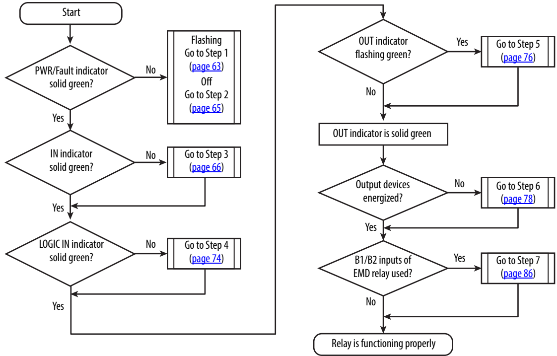
Figure 56 - Troubleshooting Flowchart
