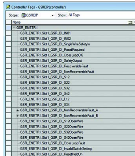
Figure 55 - AOP for the DI Safety Relay
