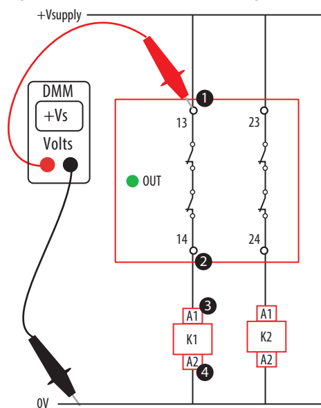
Figure 75 - Measure the Terminal Voltage
