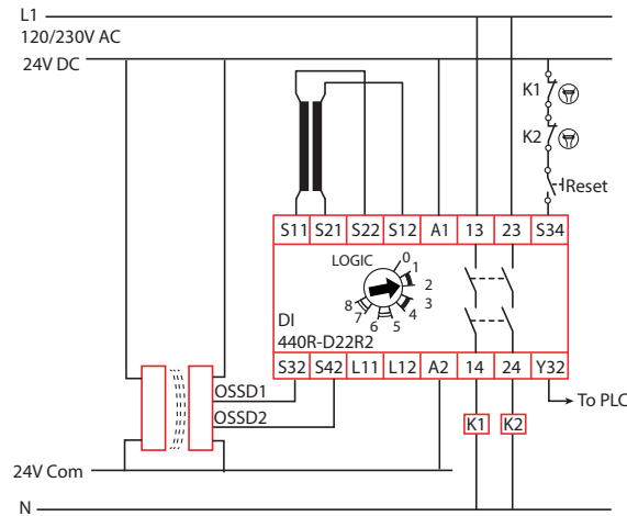
Figure 45 - With a Safety Mat and Device with OSSD Outputs, Monitored Manual Reset, AC Loads
