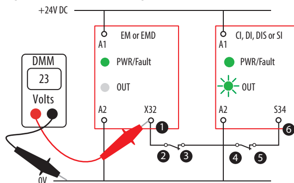
Figure 85 - Measure X32 Voltage
