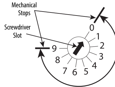
Figure 25 - Configuration Switch Adjustment
