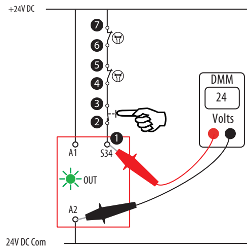
Figure 73 - Measure Reset/Monitoring Circuit Voltage
