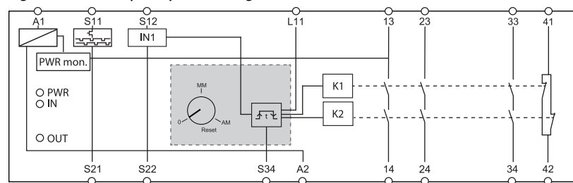
Figure 36 - CI Safety Relay Circuit Diagram
