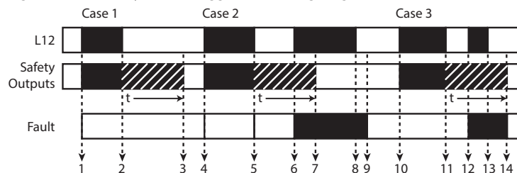
Figure 32 - Off-delay, Non-retriggerable Timing Diagram
