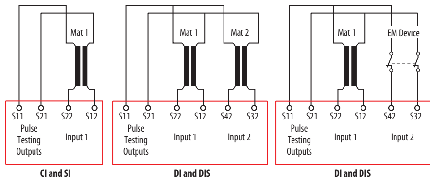
Figure 12 - Example Connections to Safety Mats
