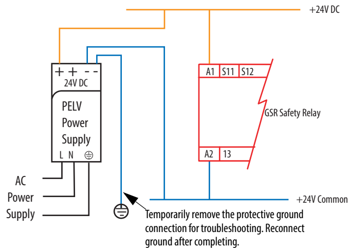
Figure 59 - 24V Common to Protective Earth Connection
