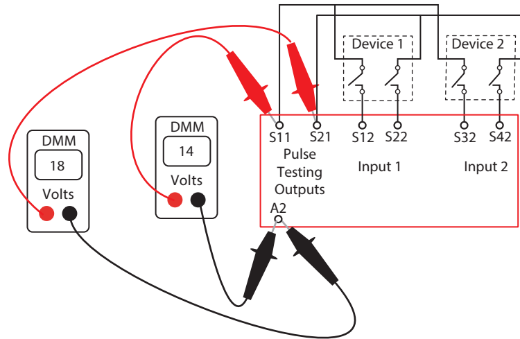
Figure 62 - Typical Voltage Measurements of the DI, DIS, and SI Relays with Contacts Open
