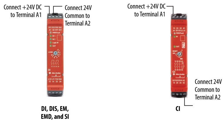
Figure 7 - Power Supply Connections
