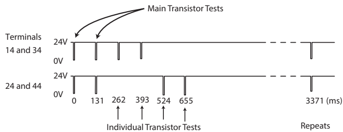
Figure 31 - OSSD Output Test Pulses on DIS Safety Relay
