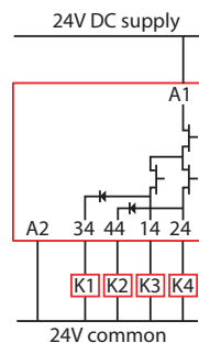
Figure 16 - OSSD Output Connections
