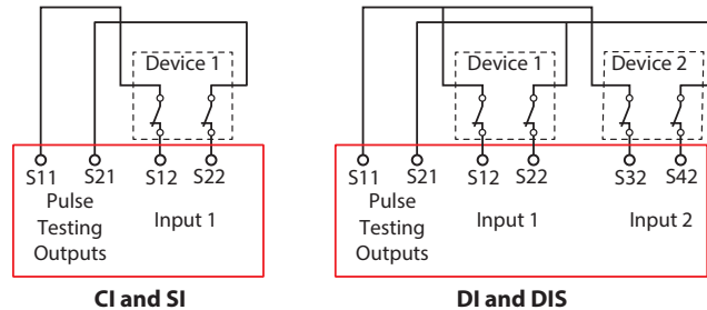
Figure 8 - Example Connections to 2 N.C. Mechanical Contacts
