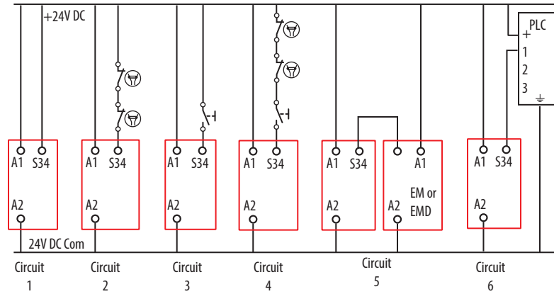
Figure 20 - Typical Reset/Monitoring Circuits
