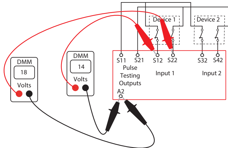
Figure 63 - Typical Voltage Measurements of the DI, DIS, and SI Relays with Contacts Closed
