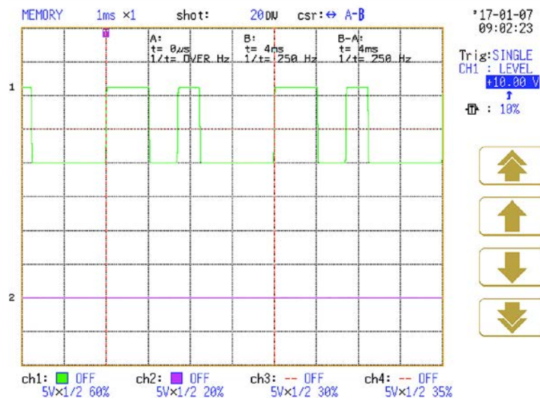
Figure 86 - The B1-B2 Waveform When the EMD Output is ON
