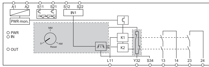
Figure 41 - SI Safety Relay Circuit Diagram
