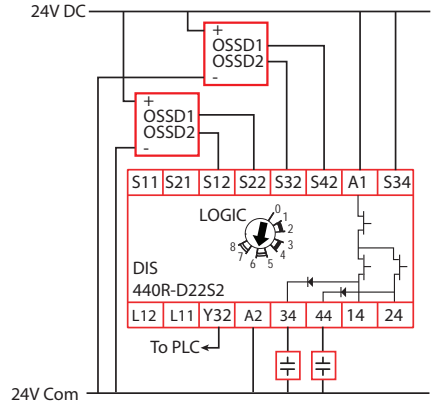
Figure 47 - High Capacitive Load
