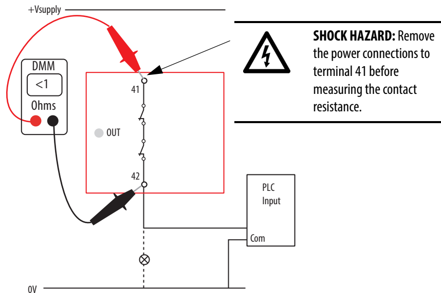
Figure 83 - Measure Contact Resistance of Aux Output Terminals
