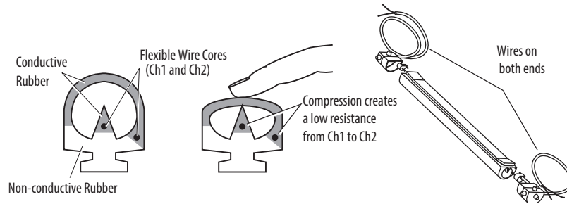
Figure 13 - Safedge Operating Principle
