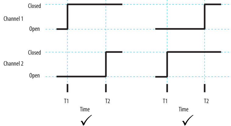
Figure 68 - GSR Relays Have Infinite Simultaneity (Discrepancy)
