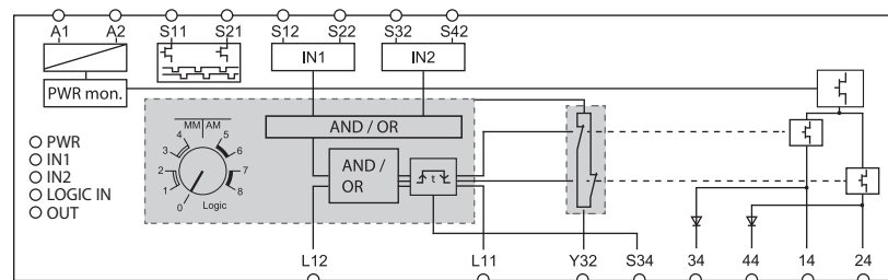
Figure 38 - DIS Safety Relay Circuit Diagram
