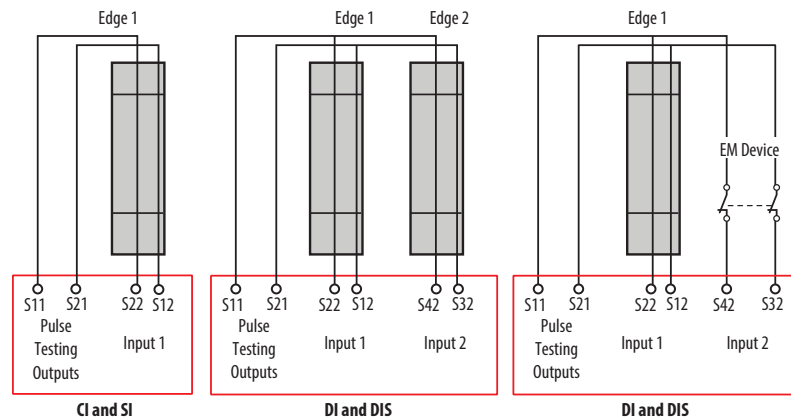
Figure 14 - Example Connections to Safety Edges
