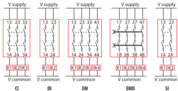
Figure 15 - Electromechanical Output Connections
