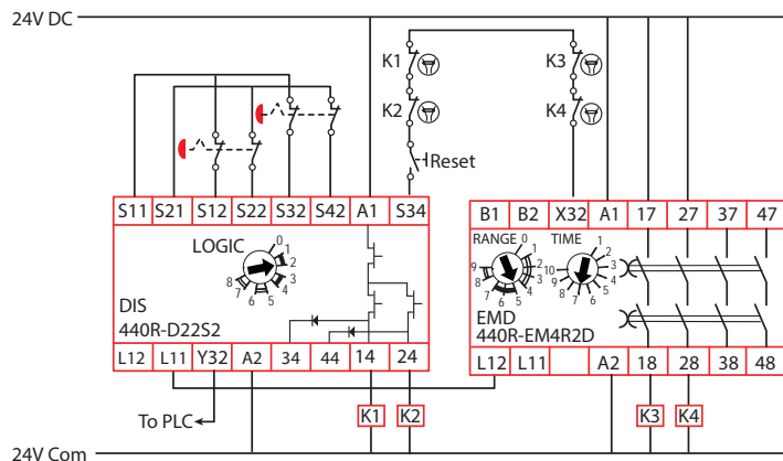
Figure 50 - EMD - On Delay
