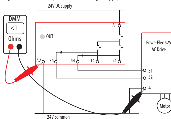
Figure 79 - Continuity Test of the Voltage Supply Common Connection
