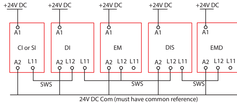
Figure 71 - Example SWS Connections
