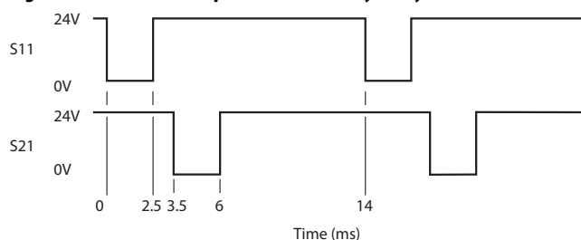
Figure 28 - Pulse Test Sequence for CI Safety Relay
