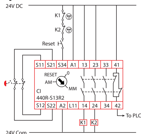
Figure 42 - Mechanical Contacts with Monitored Manual Reset
