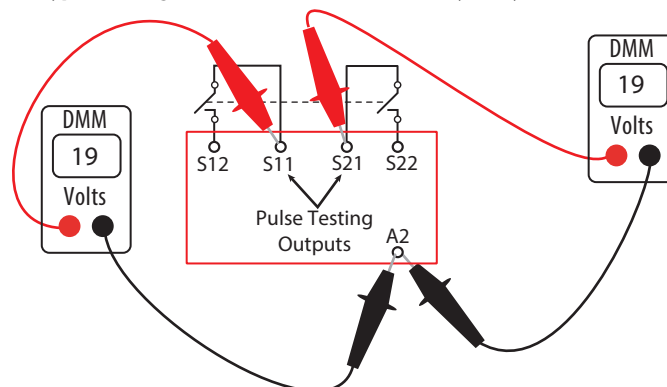
Figure 60 - Typical Voltage Measurements of the CI Safety Relay
