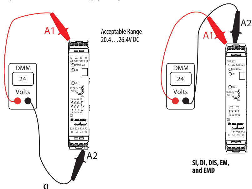
Figure 58 - Measure Power Supply Voltage
