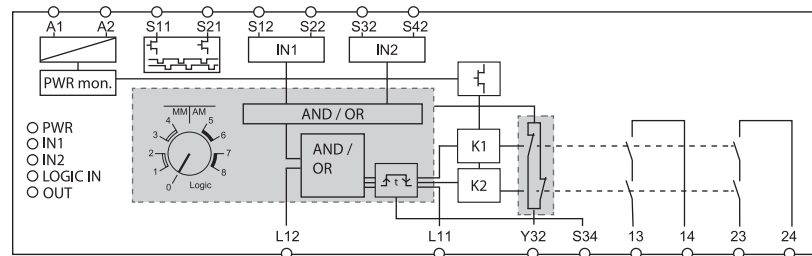
Figure 37 - DI Safety Relay Circuit Diagram
