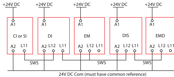
Figure 18 - Example SWS Connections
