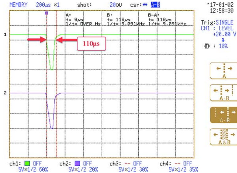
Figure 81 - OSSD Channel Transistor Test Pulse
