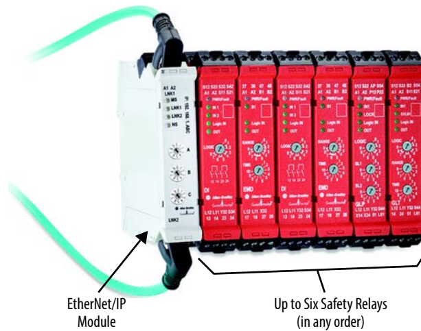
Figure 53 - Arrangement of EtherNet/IP Module and Safety Relays
