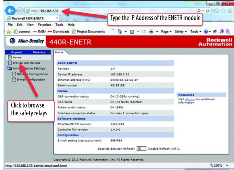
Figure 54 - ENETR Web Page
