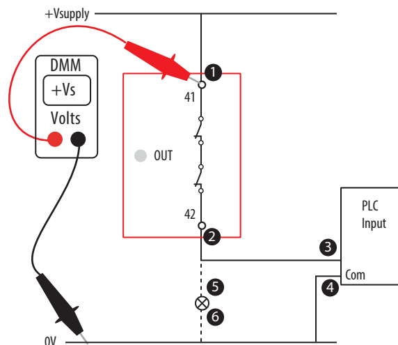
Figure 82 - Measure Voltage Aux Output Terminals
