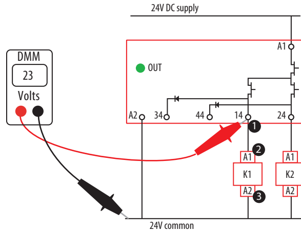
Figure 77 - OSSD Output Connections
