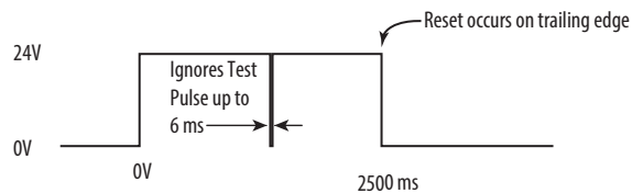
Figure 74 - Reset Input Ignores Test Pulses up to 6 ms
