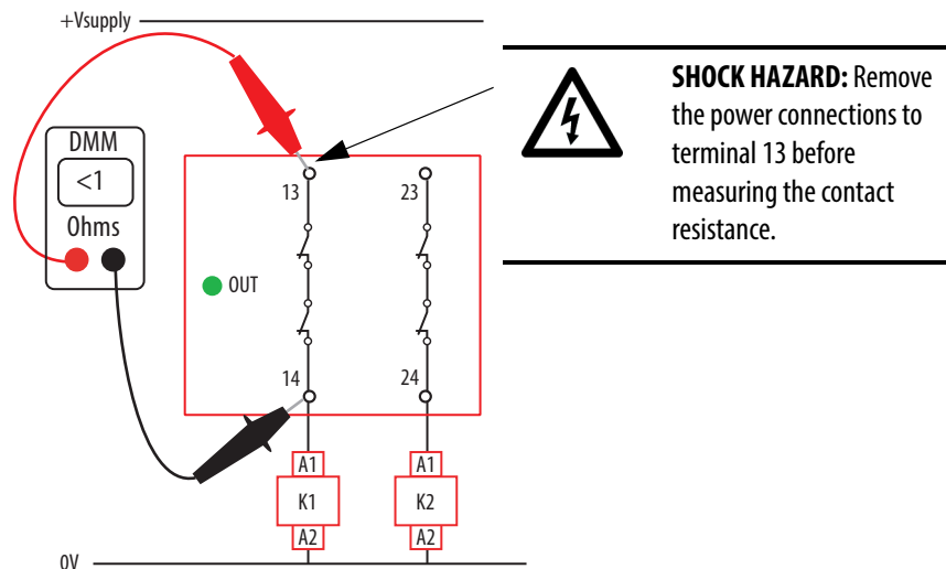
Figure 76 - Measure the Contact Resistance
