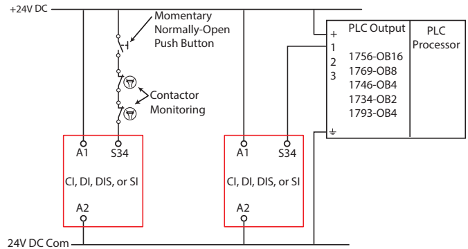
Figure 23 - Monitored Reset Connections
