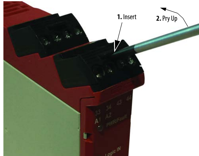
Figure 87 - Terminal Block Removal
