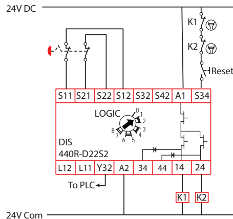
Figure 46 - Single Input, Monitored Reset
