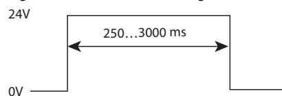
Figure 22 - Monitored Reset Signal Duration
