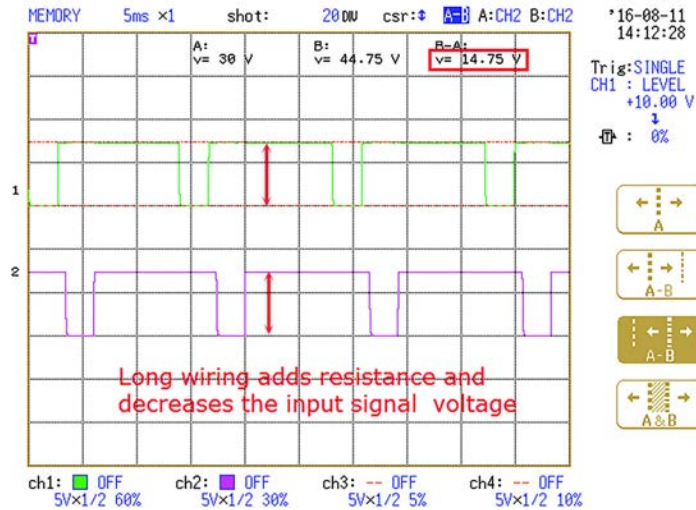
Figure 67 - Resistance Effect on Input Signal
