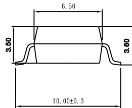
SMD Type
