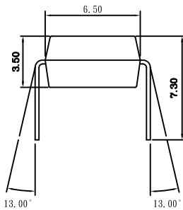
DIP Type
