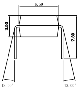
DIP Type
