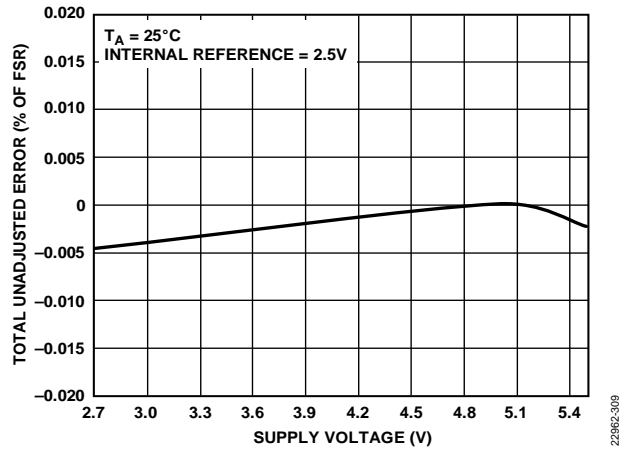
Figure 22. AD5673R Total Unadjusted Error vs. Supply Voltage
