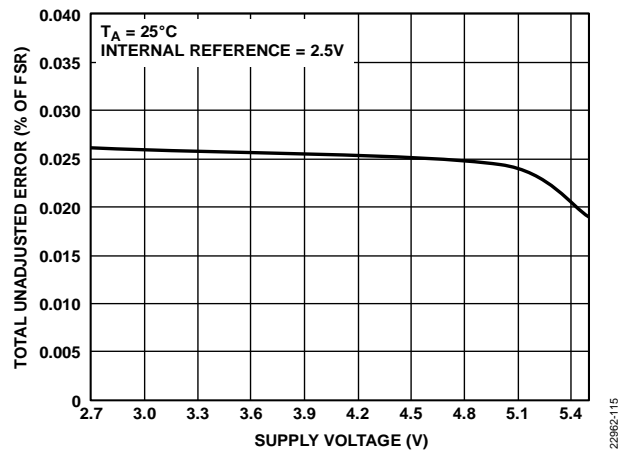
Figure 21. AD5677R Total Unadjusted Error vs. Supply Voltage
