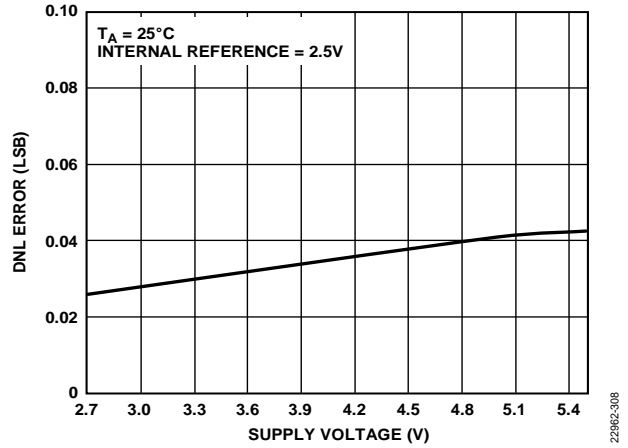
Figure 20. AD5673R DNL Error vs. Supply Voltage
