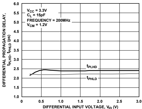
Figure 14. Differential Propagation Delay vs. Differential Input Voltage
