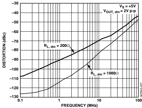
Figure 7. Second Harmonic Distortion at V_S = 5 V at Various Loads
