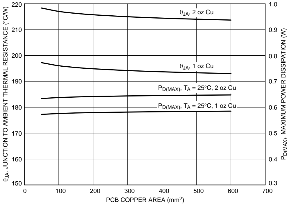
Figure 54. θ JA and P D (MAX) vs. Copper Area (XDFN44)
