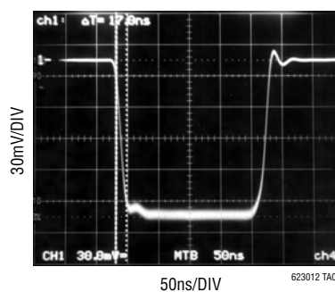
Photodiode Amplifier Time Domain Response
