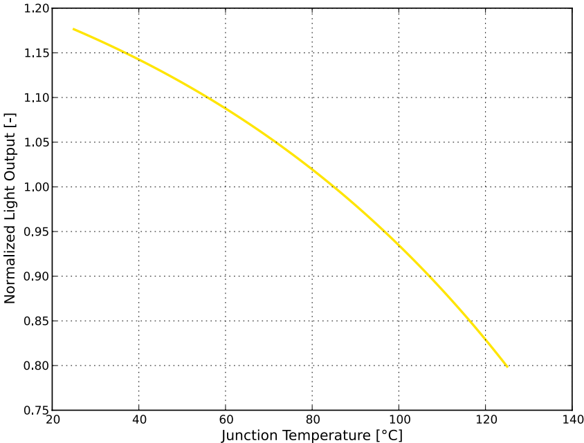
Figure 2b. Typical normalized light output vs. junction temperature for LUXEON CZ PC Amber at 350mA.
