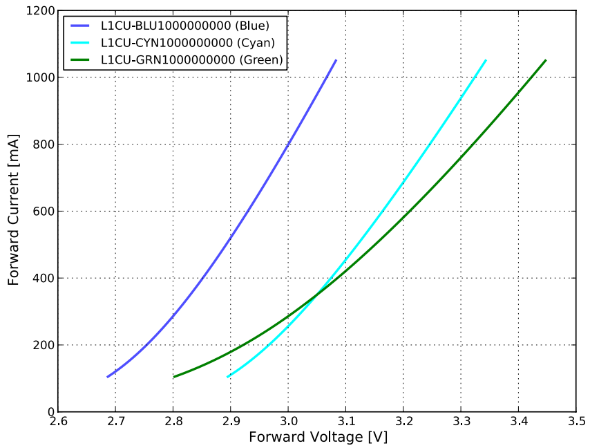
Figure 4d. Typical forward current vs. forward voltage for LUXEON CZ Green, Cyan and Blue at T_j=85^\circ\text{C} .
