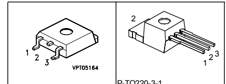
P-TO263-3-2
