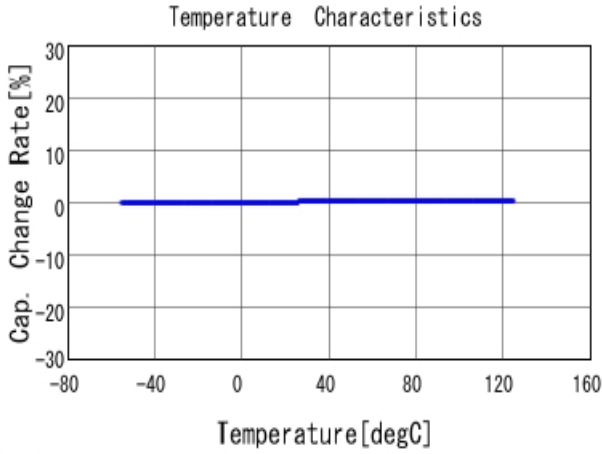
■ GRM31A5C3A101JW01 C-Temp. capchange, DCOV, AC1Vrms
