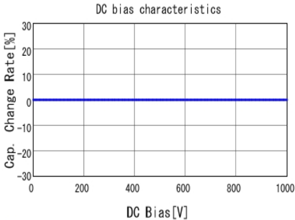
■ GRM31A5C3A101JW01 C-DC bias capchange, 25.0degC, AC1V
