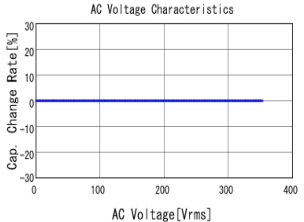
■ GRM31A5C3A101JW01 C-AC Voltage capchange, DCOV, 25.0d
