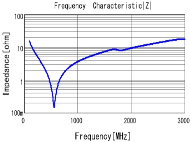
■ GRM31A5C3A101JW01 |Z| DCOV, 25degC
