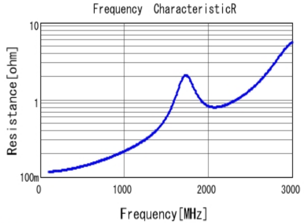
■ GRM31A5C3A101JW01 R DCOV, 25degC
