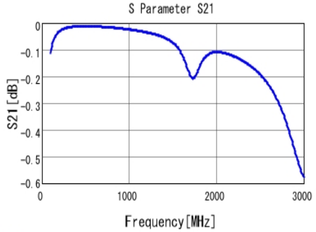
■ GRM31A5C3A101JW01 S21 DCOV, 25degC
