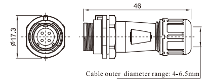
In-Line Cable Connector Mate With OL1110 (Equipped with dust cover)
