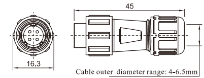
Cable Pulg Mate With OL1111, OL1112
