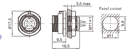
Rear-nut Socket Mate With OL1110 (Equipped with dust cover)
