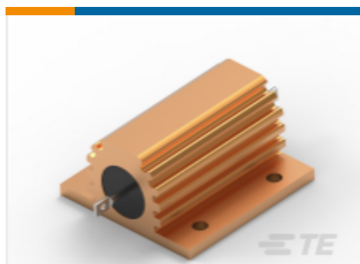
TE Part #1630012-2 Power Resistor: Aluminum Housed, HSA
