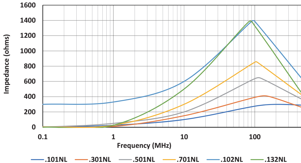
PA4339.XXXNLT, Typical Impedance versus Frequency
