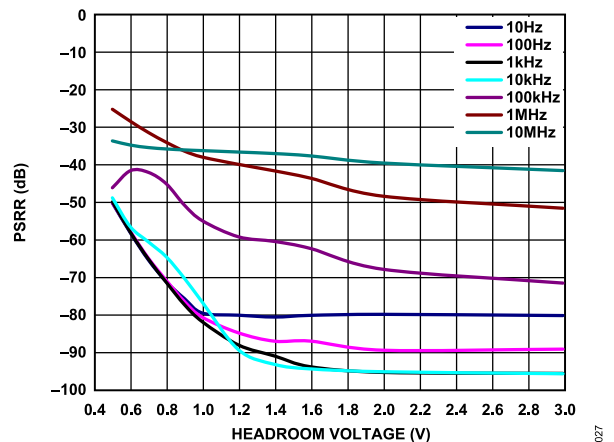
Figure 29. Power Supply Rejection Ratio (PSRR) vs. Headroom Voltage, V_{OUT} = 3.3\text{ V} , for Different Frequencies
