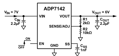
Figure 43. Typical Adjustable Output Voltage Application Schematic
