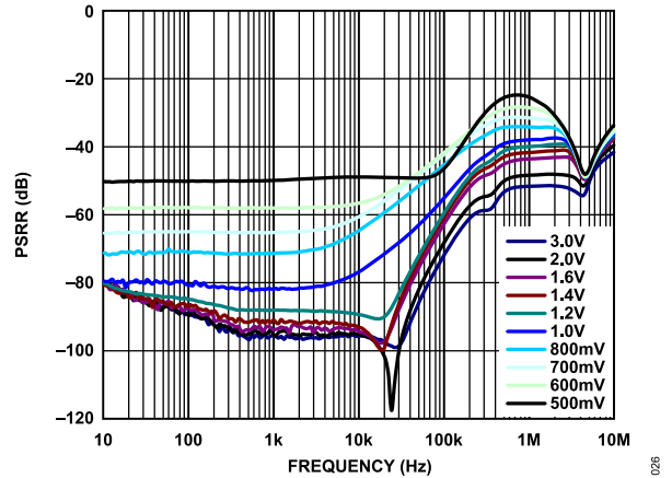
Figure 28. Power Supply Rejection Ratio (PSRR) vs. Frequency, V_{OUT} = 3.3\text{ V} , for Various Headroom Voltages
