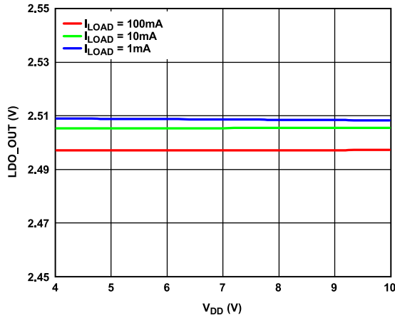
Figure 47. Output Voltage (LDO_OUT) vs. V DD
