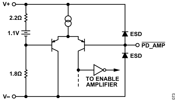
Figure 61. Shutdown Circuit
