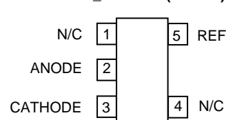
LM4041_ADJH5 (SC70-5)
