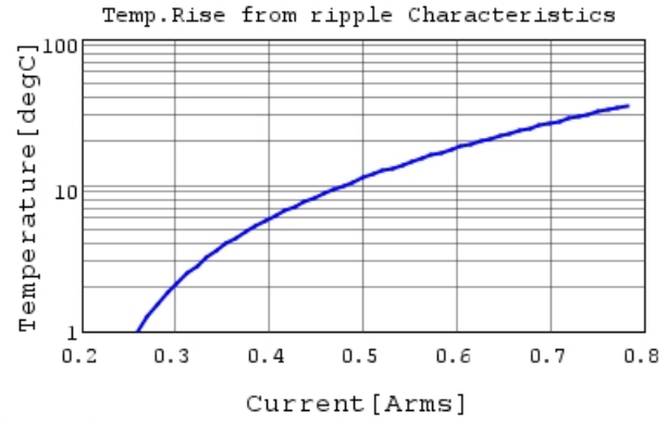
GJM1555C1H1R1CB01 Temp.rise 3GHz
