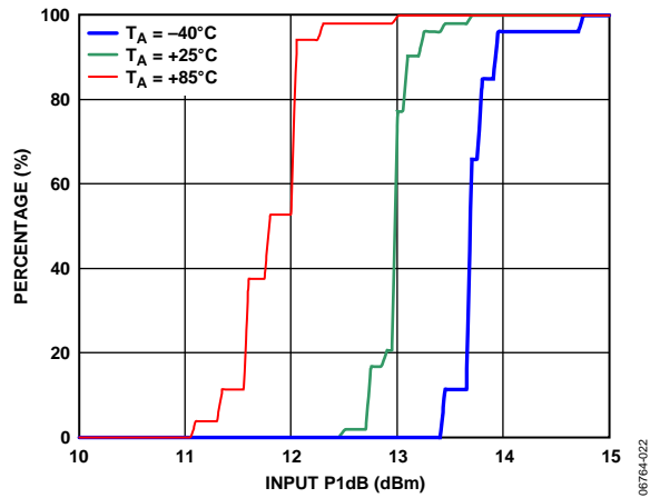
Figure 26. IP1dB Distributions
