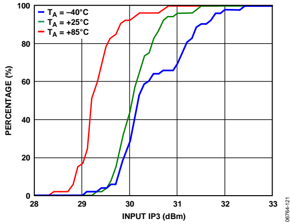
Figure 25. IIP3 Distributions
