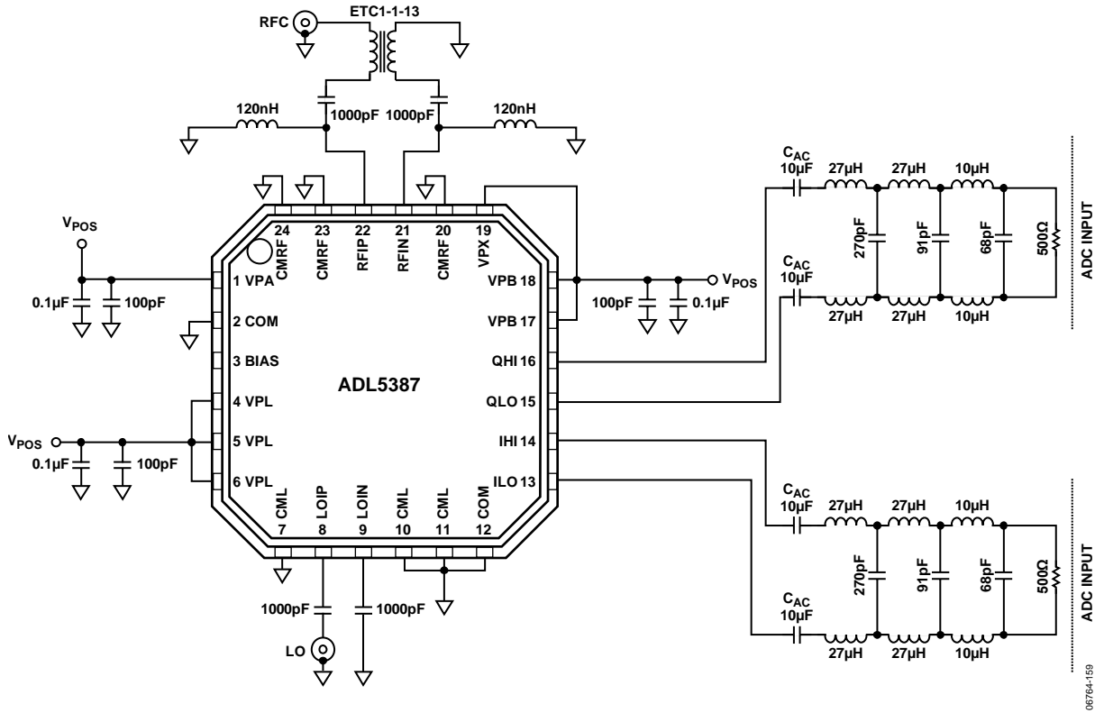
Figure 63. Sixth Order Low-Pass Butterworth Baseband Filter Schematic
