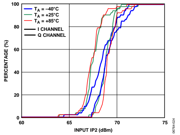
Figure 28. IIP2 Distributions for I Channel and Q Channel
