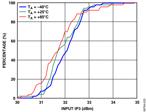
Figure 37. IIP3 Distributions
