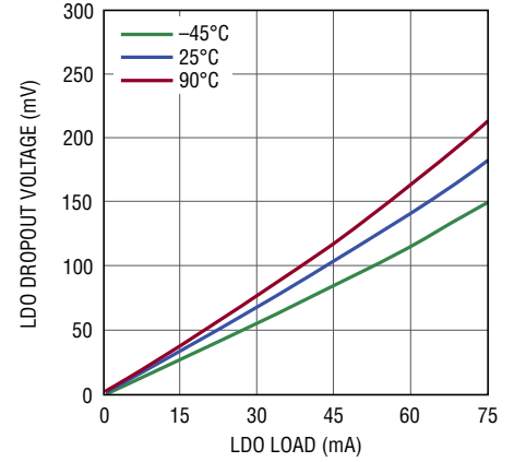
LDO Dropout Voltage at V_{INLDO} = 1.8\text{V}
