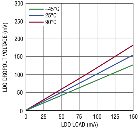
LDO Dropout Voltage at V_{INLDO} = 3.8\text{V}
