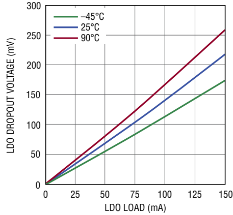
LDO Dropout Voltage at V_{INLDO} = 2.5\text{V}
