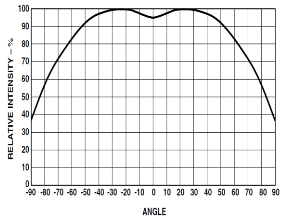
Figure 5: Radiation Pattern
