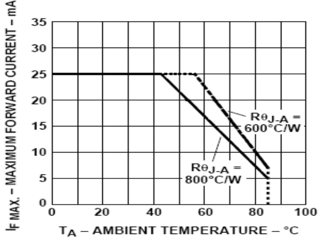
Figure 6: Derating Curve
