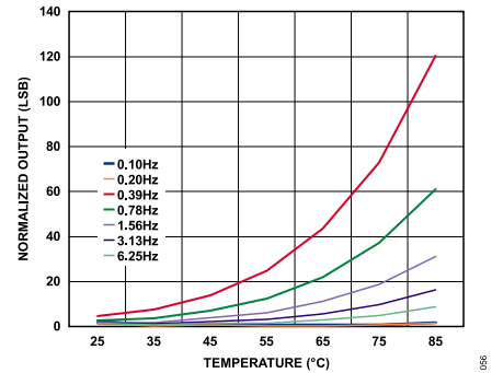
Figure 54. Typical X-Axis Output vs. Temperature at Lower Data Rates, Normalized to 100 Hz Output Data Rate, V_S = 2.5 V
