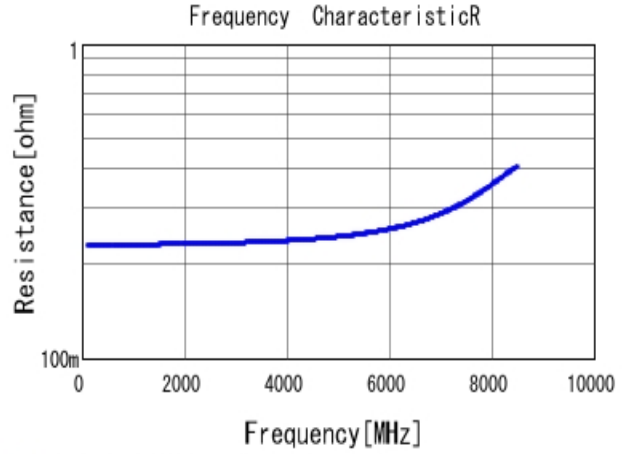
GJM1555C1H1R2BB01 R DC0V, 25degC
