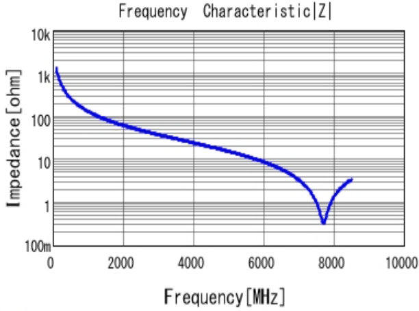
GJM1555C1H1R2BB01 |Z| DC0V, 25degC
