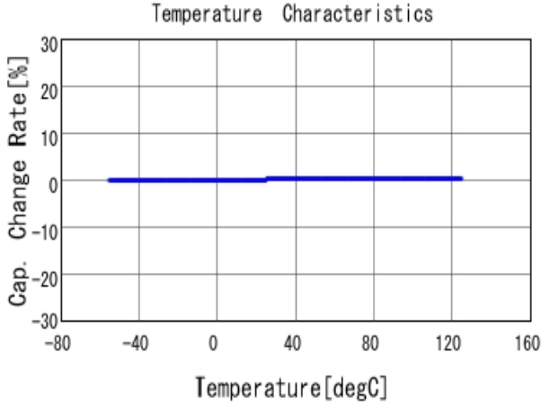
■ GJM1555C1H1R2BB01 C-Temp. capchange, DCOV, AC1Vrms
