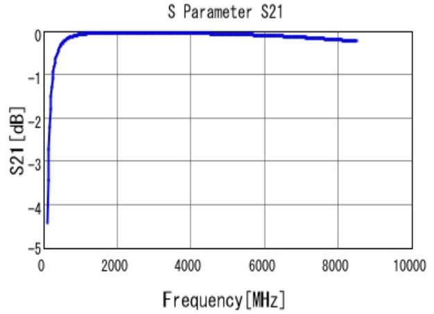
■ GRM0335C1E120JA01 S21 DCOV, 25degC
