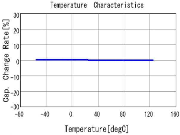
■ GRM0335C1E120JA01 C-Temp. capchange, DCOV, AC1Vrms
