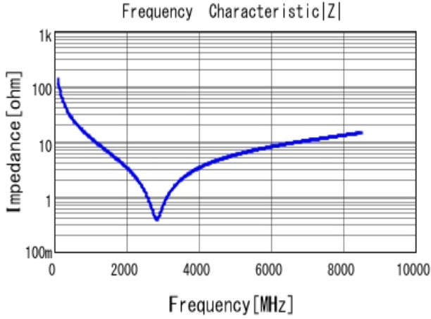
■ GRM0335C1E120JA01 |Z| DC0V, 25degC
