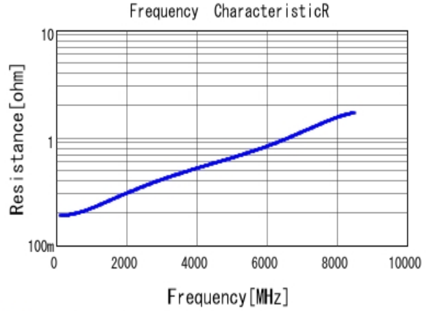
■ GRM0335C1E120JA01 R DC0V, 25degC
