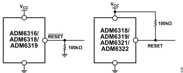
Figure 18. Ensuring Reset Valid to V_{CC} = 0\text{ V}
