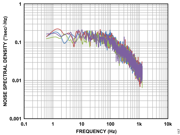
Figure 18. Typical Noise Spectral Density ( C_{OUT} = 0.01\ \mu\text{F} )
