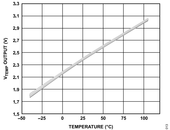
Figure 12. V_{TEMP} Output over Temperature, 256 Parts ( V_{RATIO} = 5 V )
