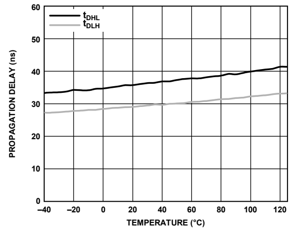
Figure 14. Propagation Delay vs. Temperature, 2 \text{ nF} Load
