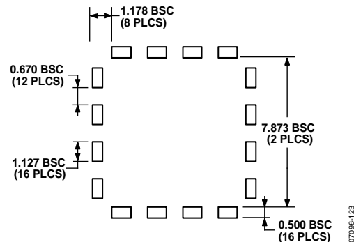
Figure 29. Example Pad Layout
