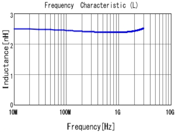
■ LQP15MN2N4W02 L
