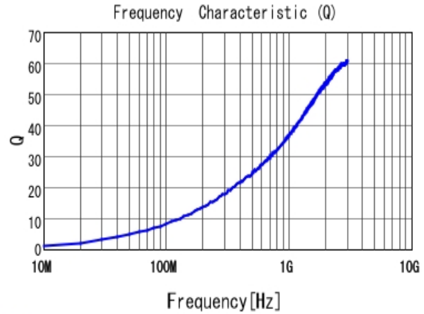
■ LQP15MN2N4W02 Q
