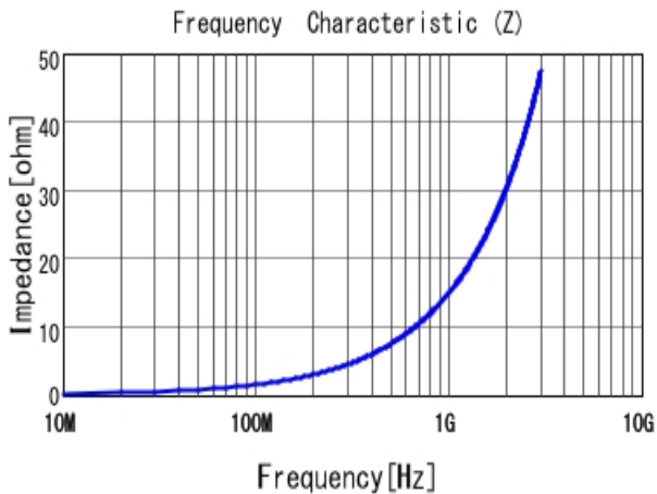
■ LQP15MN2N4W02 |Z|
