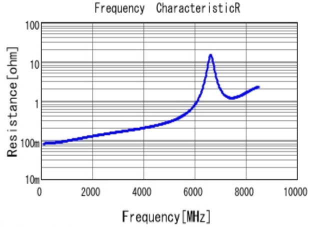
GJM1555C1H100GB01 R DC0V, 25degC
