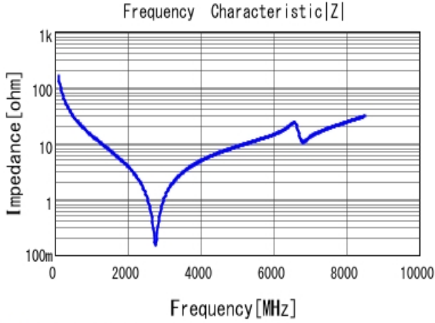
GJM1555C1H100GB01 |Z| DC0V, 25degC
