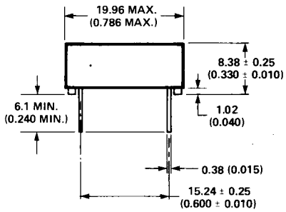
END VIEW
