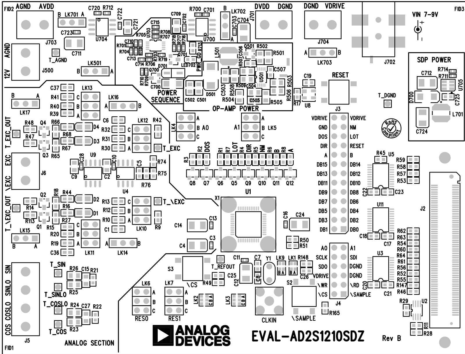
EVAL-AD2S1210SDZ (Rev. B) Top Side View.
