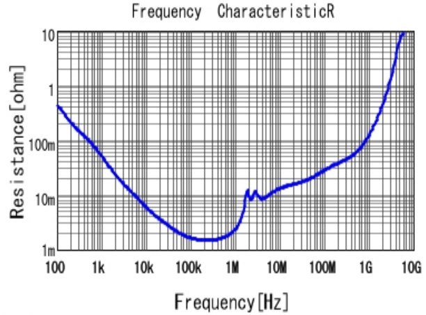
■ GRM32ER71A226ME20 R DCOV, 25degC
