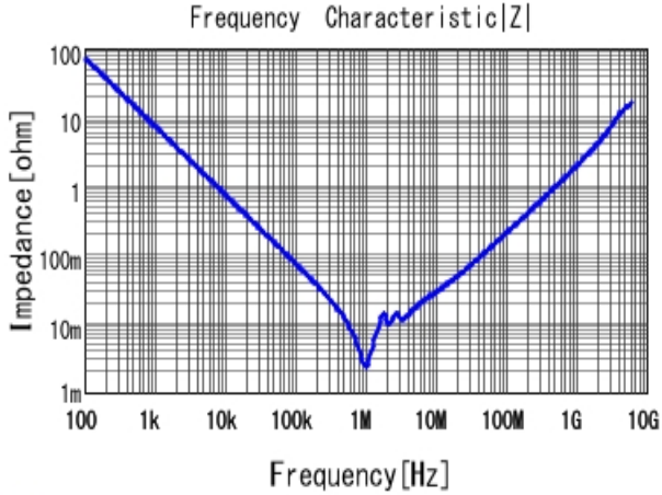
■ GRM32ER71A226ME20 |Z| DCOV, 25degC
