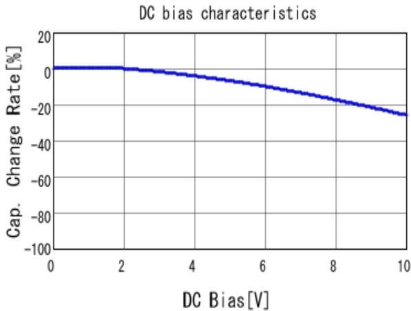
■ GRM32ER71A226ME20 C-DC bias capchange, 25.0degC, AC0.
