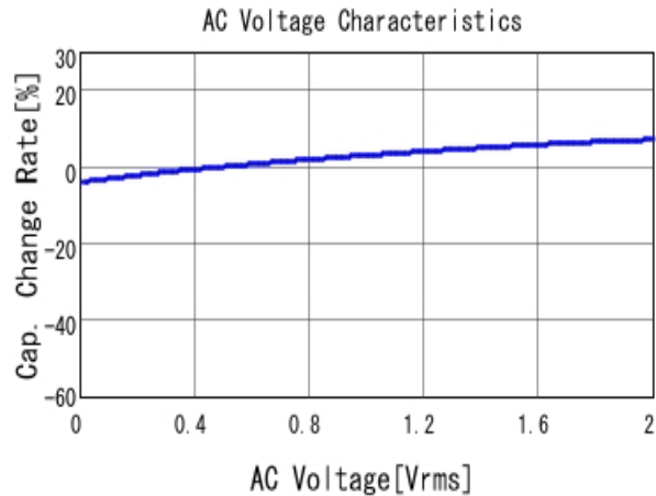
■ GRM32ER71A226ME20 C-AC Voltage capchange, DCOV, 25.0d
