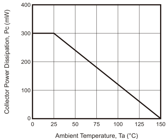
Fig.8 - P_c — T_a
