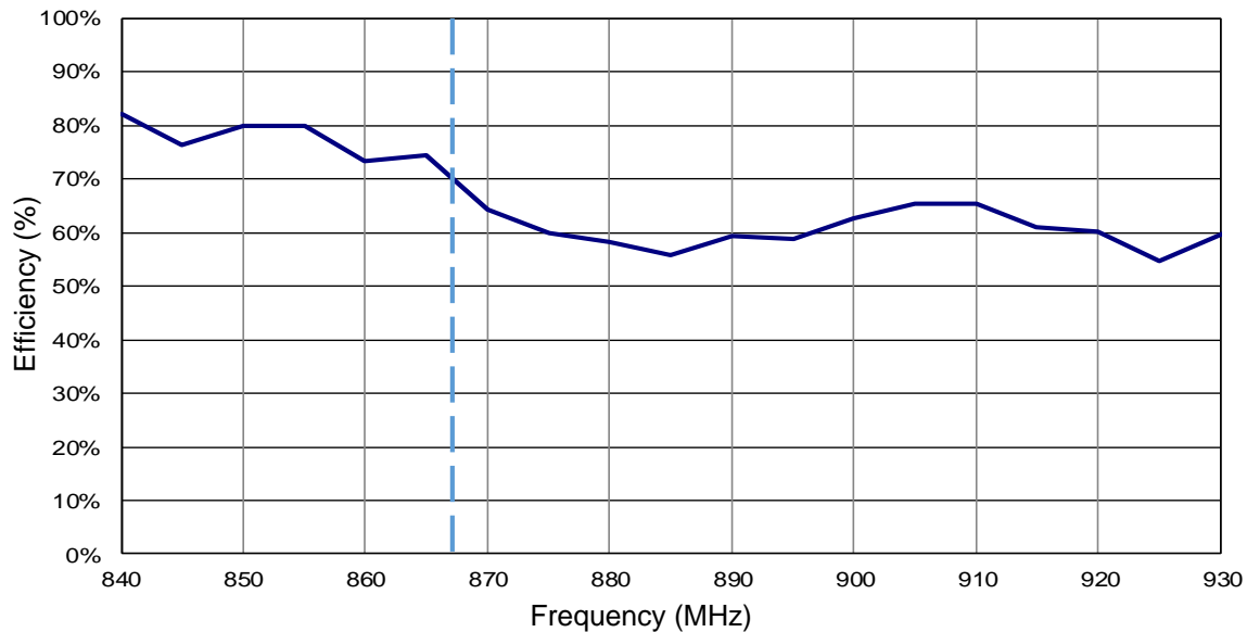
Efficiency
