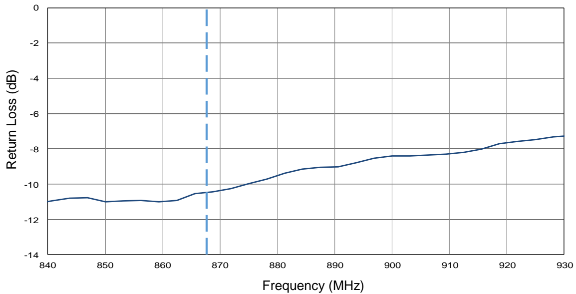
Return Loss
