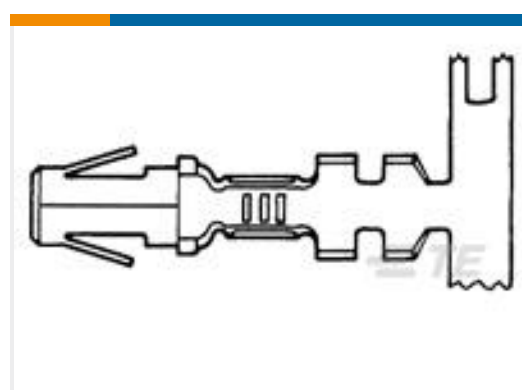
TE Part #61626-2 .140 DIA SOK 20-14 PTPPHBZ
