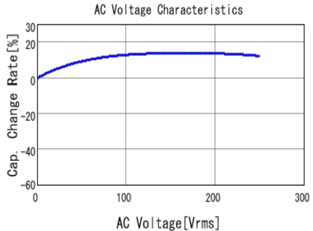
■ GA342QR7GD152KW01 C-AC Voltage capchange, DC0V, 25.0d
