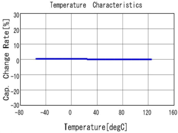
■ GRM0335C1H8R2DA01 C-Temp. capchange, DCOV, AC1Vrms
