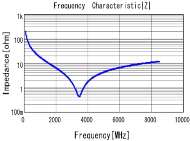
■ GRM0335C1H8R2DA01 |Z| DCOV, 25degC
