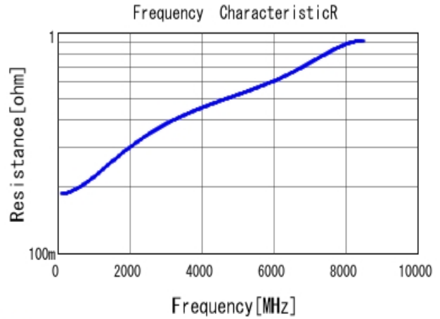
■ GRM0335C1H8R2DA01 R DCOV, 25degC
