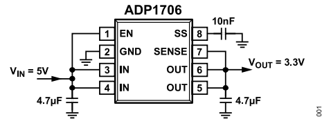
Figure 1. ADP1706 with Fixed Output Voltage, 3.3 V
