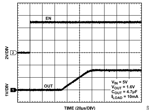
Figure 29. OUT Ramp-Up with Internal Soft Start
