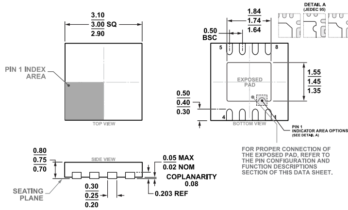
Figure 44. 8-Lead Frame Chip Scale Package [LFCSP] 3 mm x 3 mm Body and 0.75 mm Package Height (CP-8-13) Dimensions shown in millimeters
