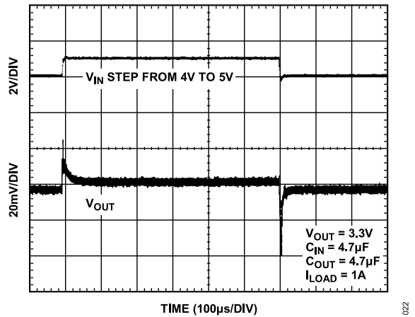
Figure 21. Line Transient Response
