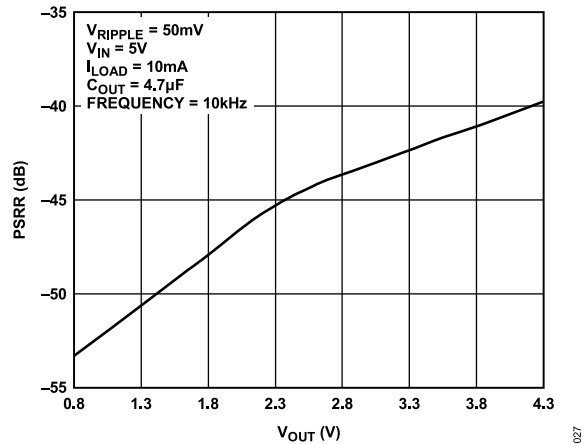
Figure 26. ADP1708 Power Supply Rejection Ratio (PSRR) vs. Output Voltage ( V_{OUT} )
