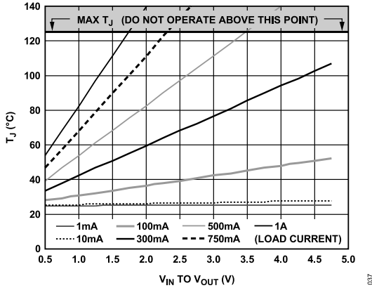
Figure 38. 0 mm 2 of PCB Copper, T A = 25°C, SOIC
