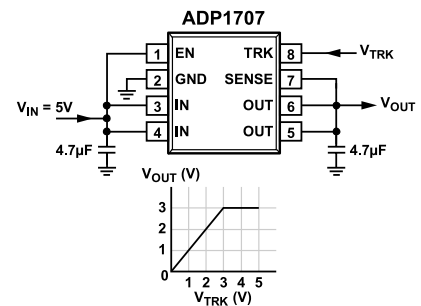
Figure 2. ADP1707 with Output Voltage Tracking
