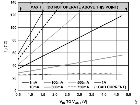
Figure 41. 0 mm 2 of PCB Copper, T A = 25°C, LFCSP
