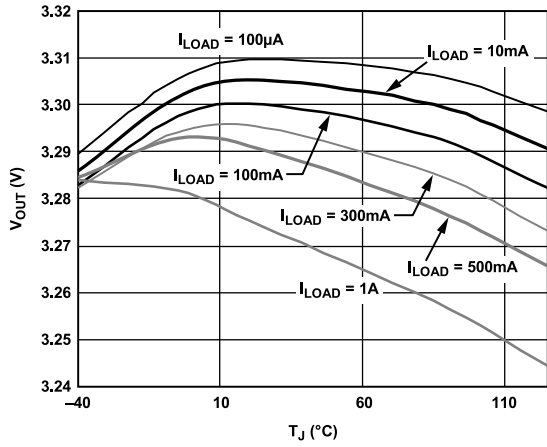
Figure 10. Output Voltage ( V_{OUT} ) vs. Junction Temperature ( T_J )
