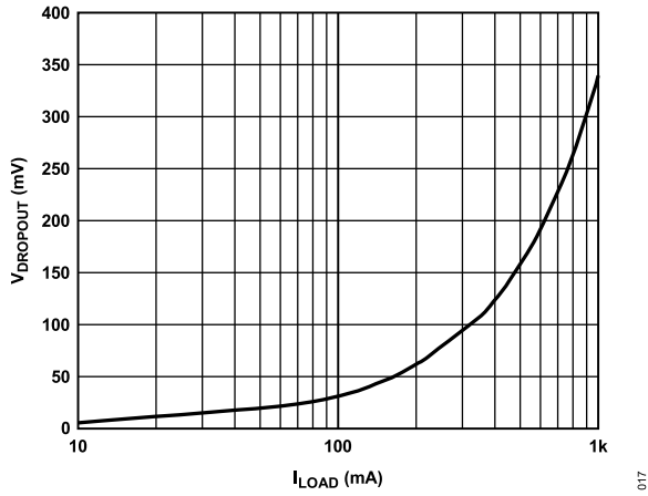
Figure 16. Dropout Voltage ( V_{DROP} ) vs. Load Current ( I_{LOAD} )
