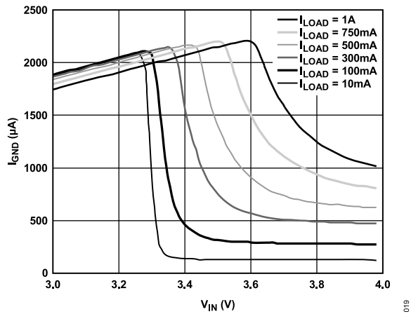
Figure 18. Ground Current ( I_{GND} ) vs. Input Voltage ( V_{IN} ) (in Dropout)
