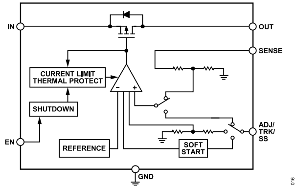
Figure 27. Internal Block Diagram
