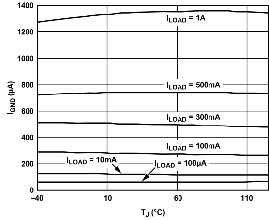
Figure 13. Ground Current ( I_{GND} ) vs. Junction Temperature ( T_J )
