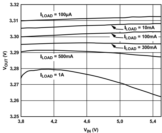
Figure 12. Output Voltage ( V_{OUT} ) vs. Input Voltage ( V_{IN} )
