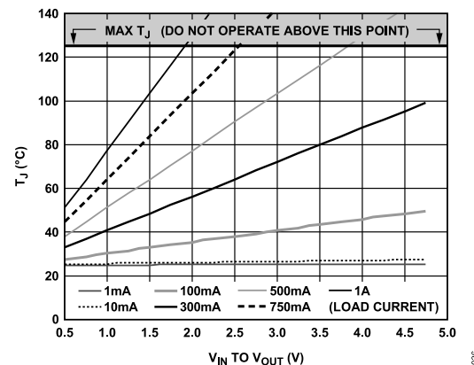
Figure 37. 100 mm 2 of PCB Copper, T_A = 25^\circ\text{C} , SOIC
