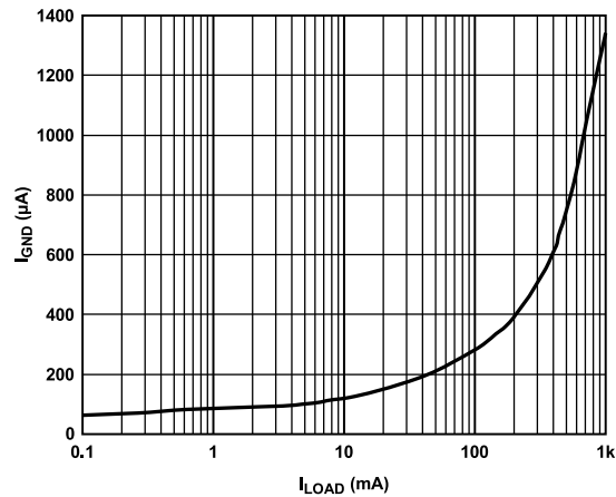
Figure 14. Ground Current ( I_{GND} ) vs. Load Current ( I_{LOAD} )
