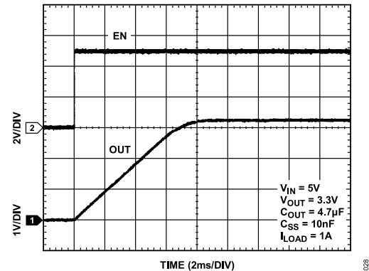
Figure 28. OUT Ramp-Up with External Soft Start Capacitor
