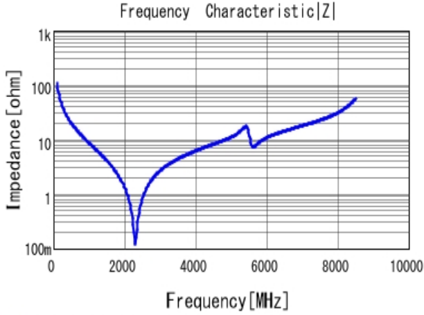
■ GJM1555C1H150GB01 |Z| DC0V, 25degC
