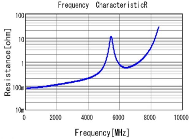
■ GJM1555C1H150GB01 R DC0V, 25degC
