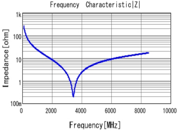
GJM1555C1H6R2WB01 |Z| DC0V, 25degC
